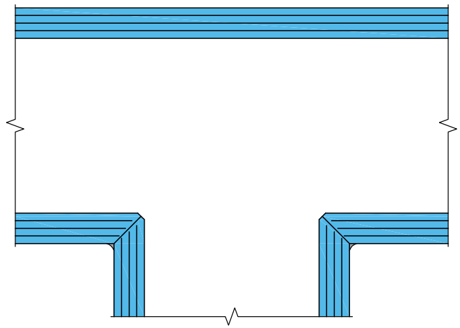
THREE WAY MINIMAL SILICONE BEAD
