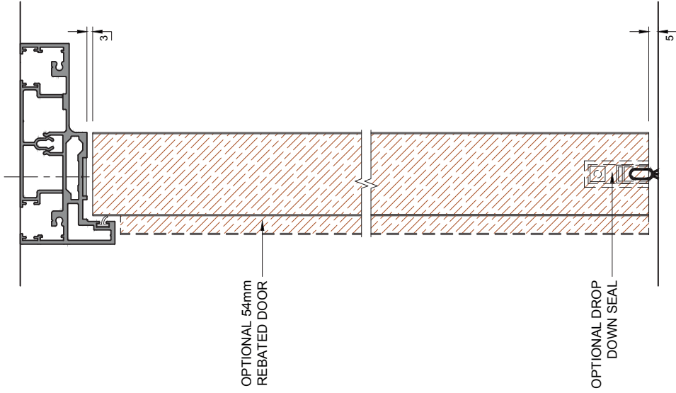
FULL HEIGHT DOOR FRAME (12mm DOOR STOP) WITH OPTIONAL 54mm REBATED DOOR
