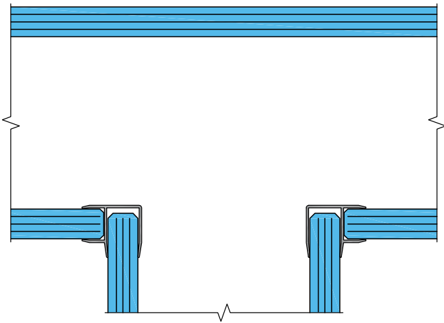
THREE WAY H-JOINT
