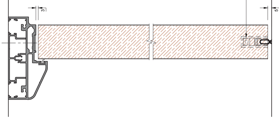
FULL HEIGHT CHAMFERED DOOR FRAME
